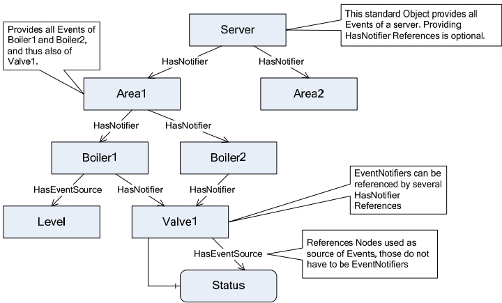
Fig. 2.45 Hierarchy of EventNotifiers
