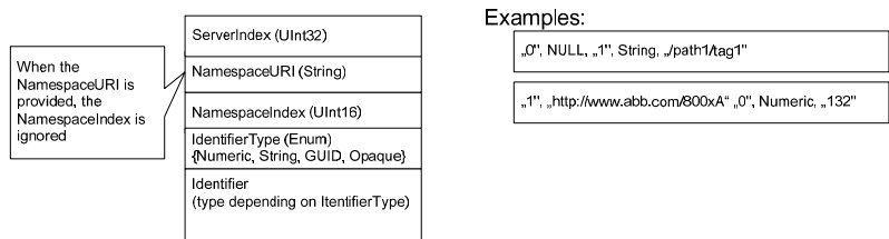
Fig. 2.37 Structure of ExpandedNodeId
