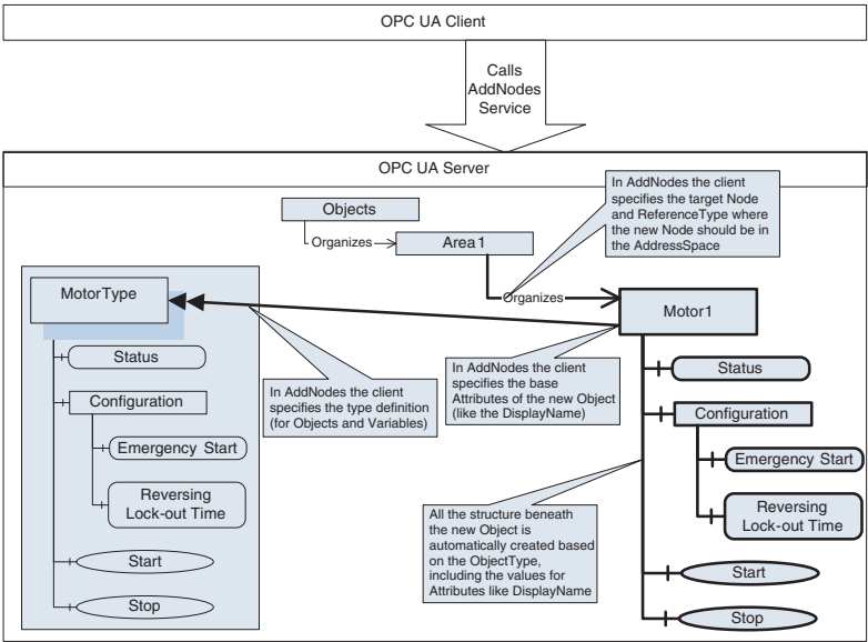
Fig. 2.16 Creating Instances based on complex ObjectTypes
