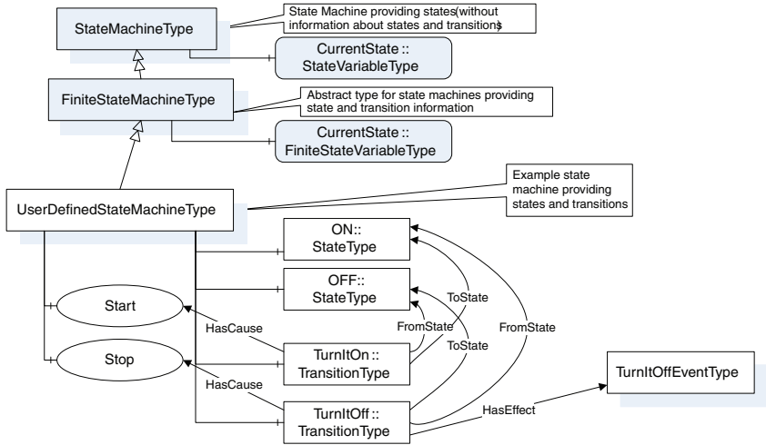
Fig. 4.7 State machine information model
