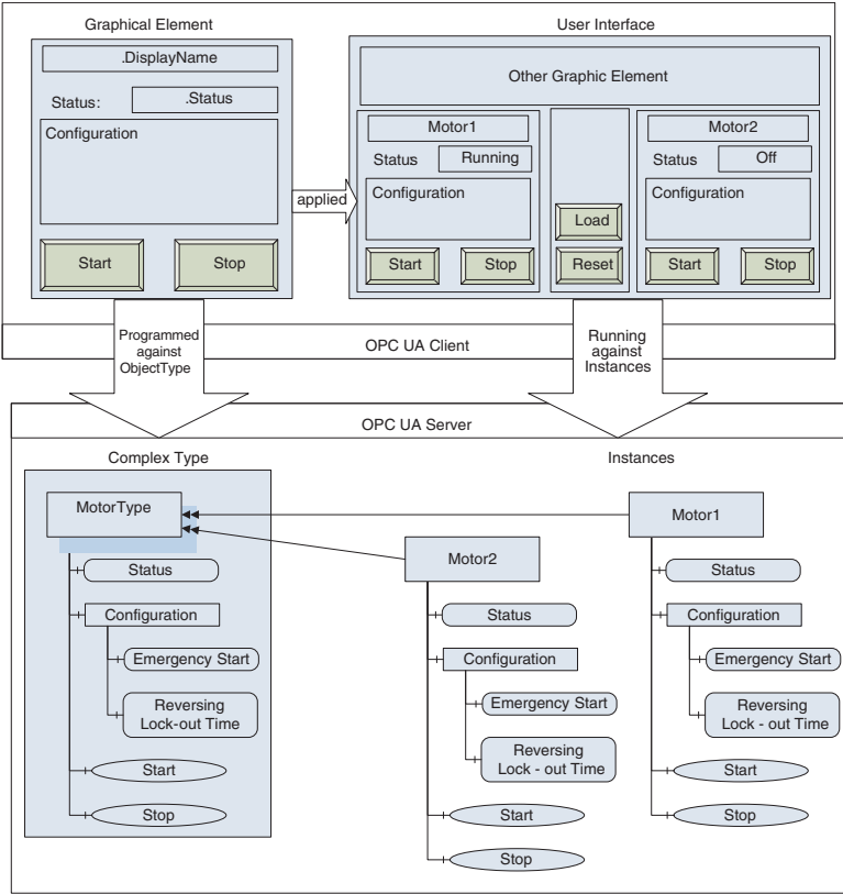
Fig. 2.15 Programming against complex ObjectType
