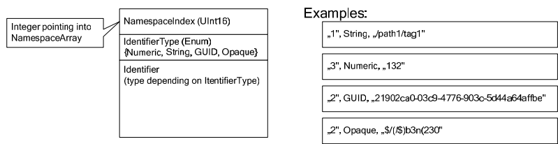
Fig. 2.35 Structure of NodeId
