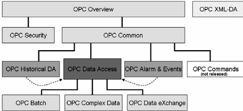
Fig. 1.5 Classic OPC interface standards
