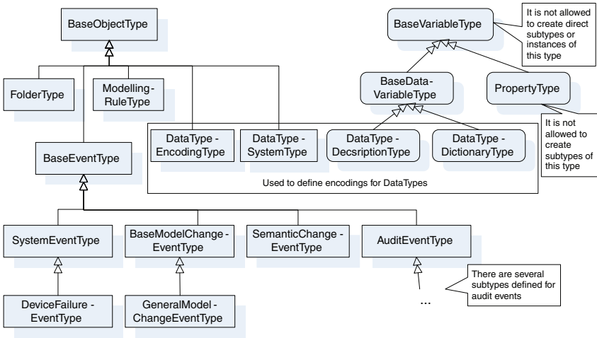
Fig. 4.1 Base TypeDefinitions
