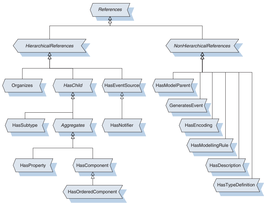
Fig. C.1 ReferenceType Hierarchy
