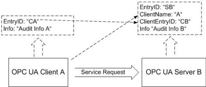
Fig. 9.15 Client–Server auditing
