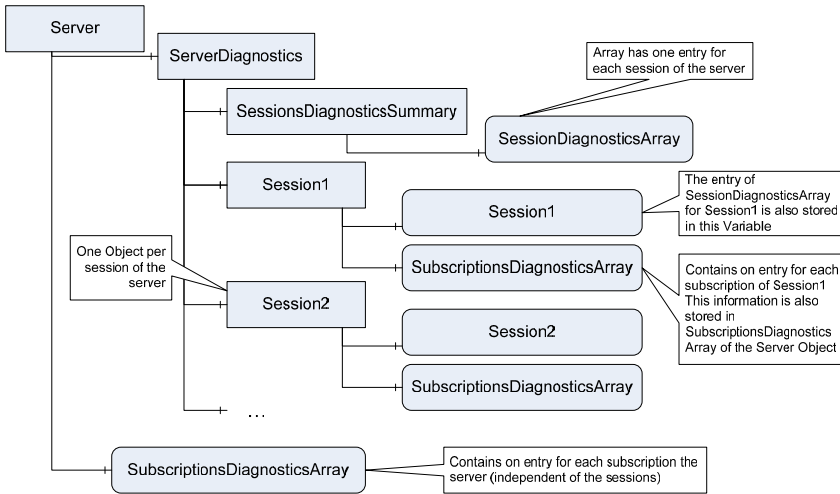
Fig. 4.4 Diagnostic information
