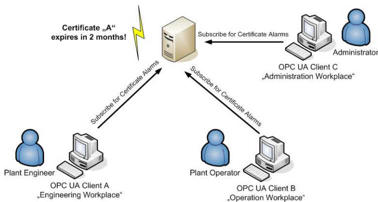
Fig. 7.24 Certificate alarms
