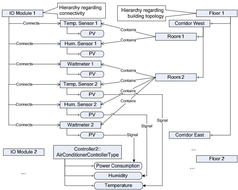
Fig. 3.7 Devices in the Address Space
