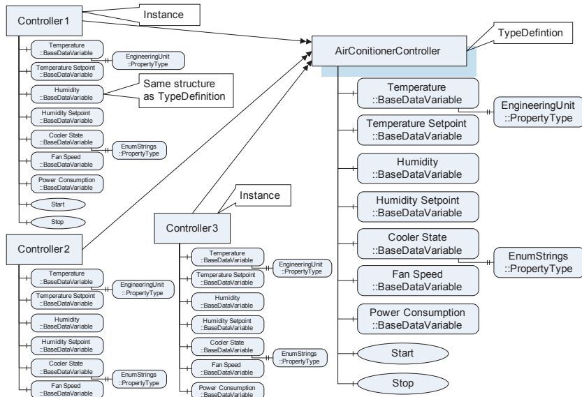
Fig. 3.4 TypeDefinition for the controller
