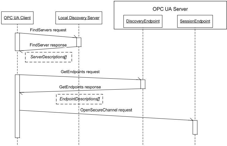
Fig. 9.11 Normal discovery
