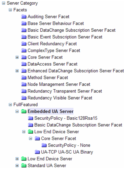
Fig. 12.2 Server-related profiles
