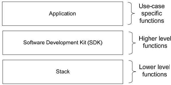
Fig. 8.1 Architectural overview
