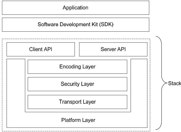
Fig. 8.2 Stack overview
