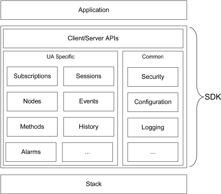
Fig. 8.3 SDK overview
