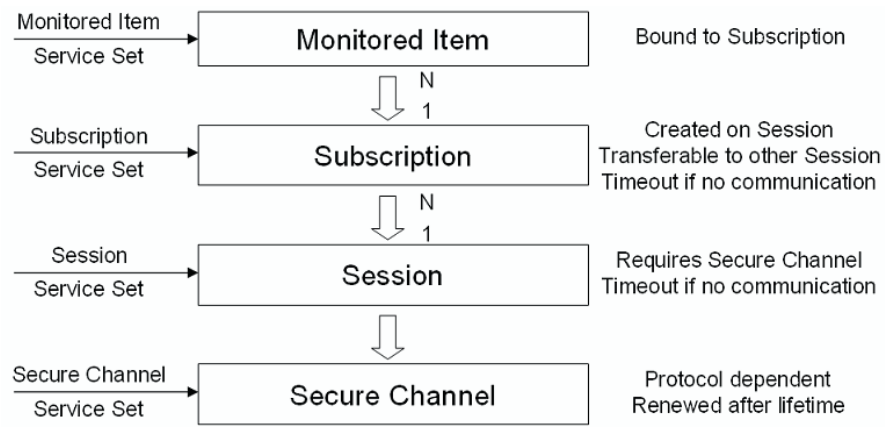
Fig. 5.2 Communication context
