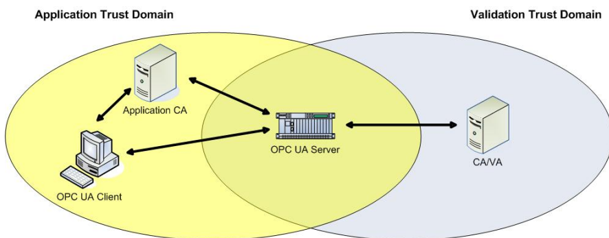
Fig. 7.28 Outsourcing certificate validation
