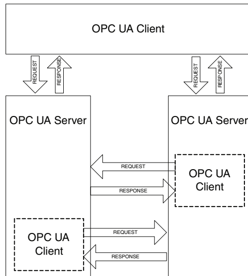
Fig. 9.4 Server-to-Server pattern
