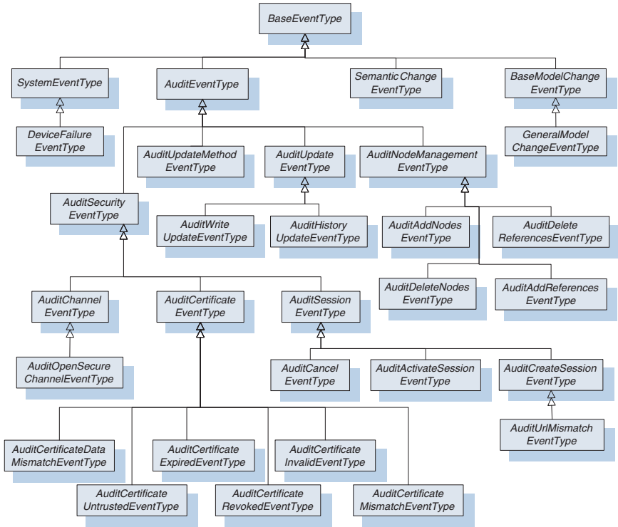
Fig. C.3 EventType Hierarchy
