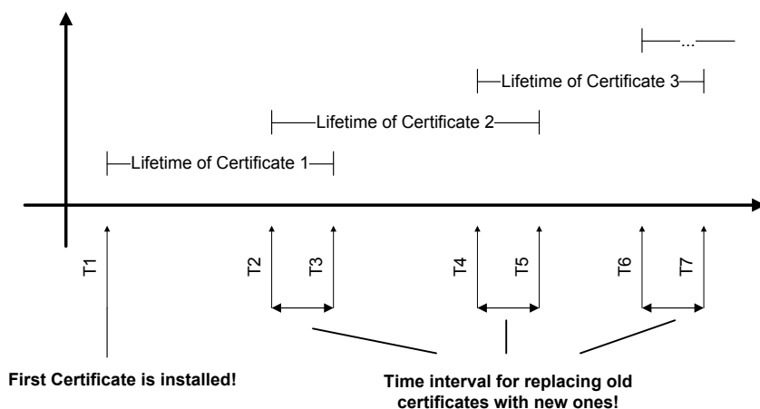
Fig. 7.25 Managing certificate renewal
